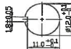
Mounting Hole
