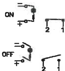
Nylon #66, Black SPST OFF-ON
