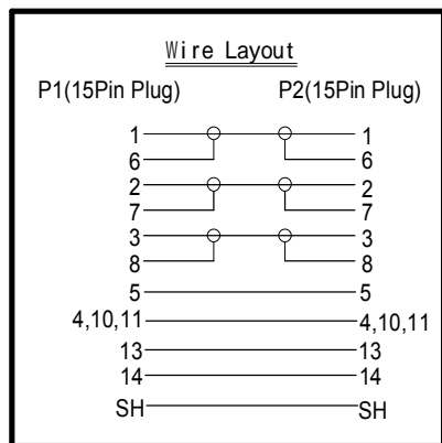
3+4 Computer cable
