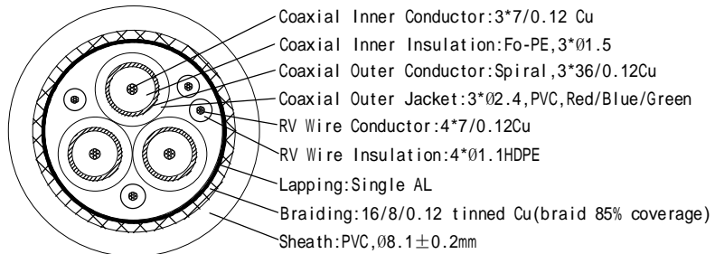
3+4 Computer cable
