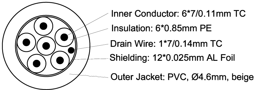
Cable Structure
