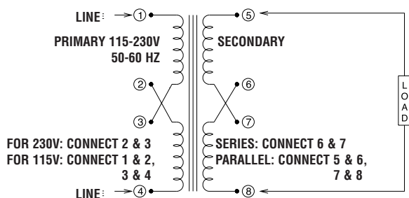
Schematic 1
