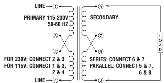
Schematic 2
